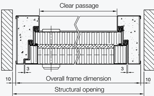
Horizontal section Single-leaf door
