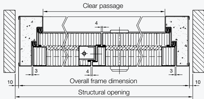
Horizontal section Double-leaf door
