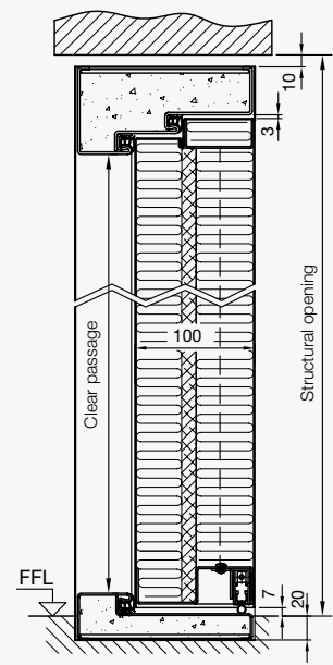
Vertical section
